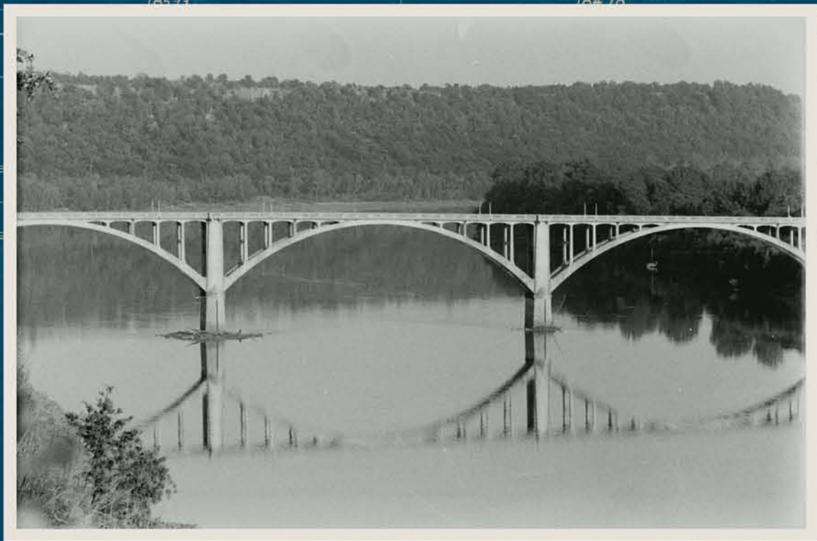
Arkansas River Bridge at Ozark, 1961.
